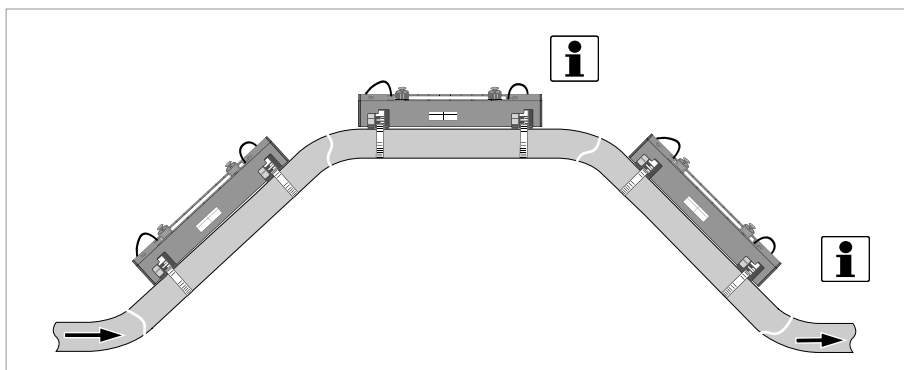
Figure 3-7: Mounting on ascending or descending pipelines is possible
