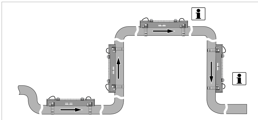
Figure 3-6: Mounting on vertical pipelines is possible
