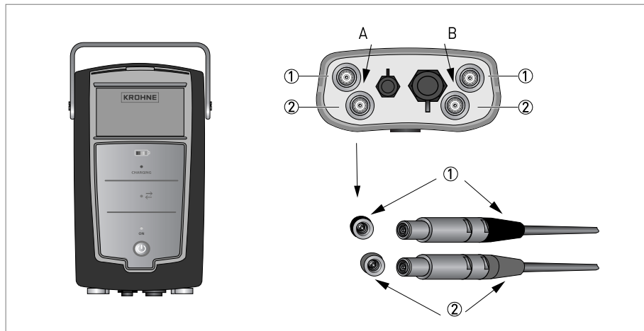
Figure 4-2: Connecting signal cables channel A and B
